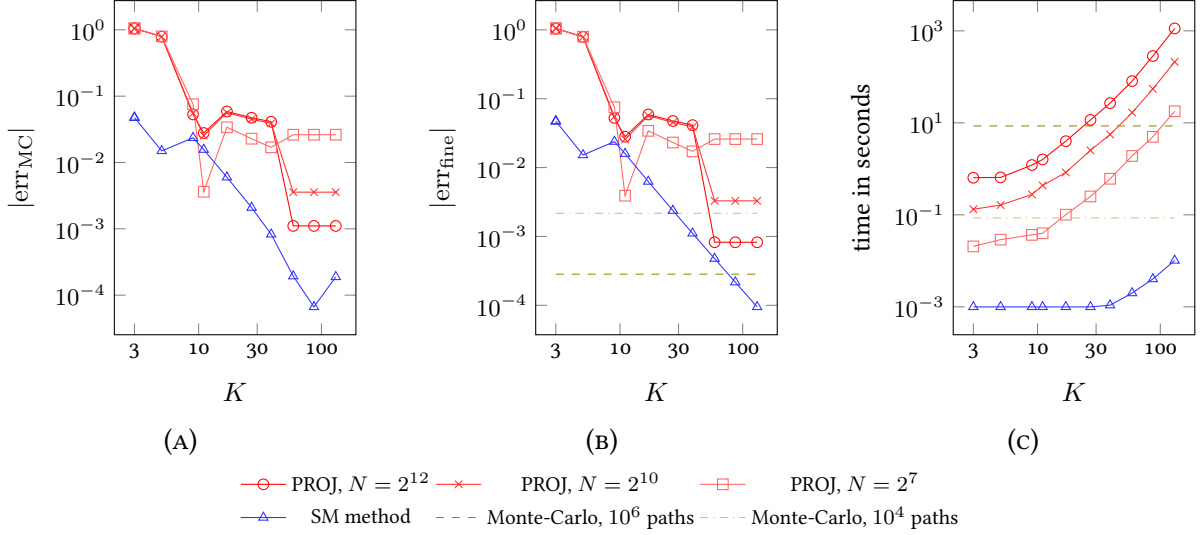
FIGURE 2. Comparison of absolute error and computation time between the SM method, the PROJ method for different values of N , and Monte-Carlo simulations. The parameters have been chosen as in Table 1.
