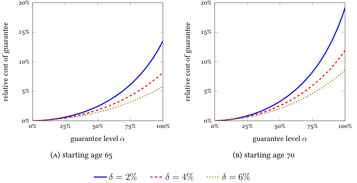
FIGURE 4. Cost of the guarantee level \alpha for different ages at contract initiation. Values are given as a relative markup in comparison with a tontine without guarantee, i.e. \alpha = 0\% .
