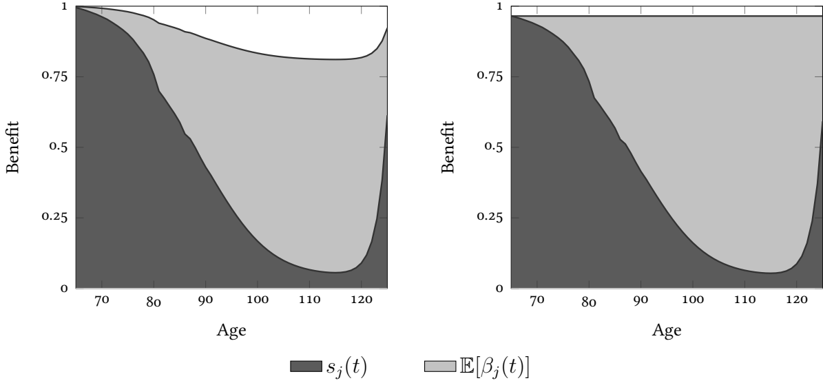
FIGURE 3. Expected future payments for a policyholder with guarantee level \alpha = 100\% after a mortality shock with (right) and without (left) update of the withdrawal schedule. The mortality shock is assumed to lead to new death probabilities \tilde{q}_{x_j+t} = 0.8 \cdot q_{x_j+t} .
