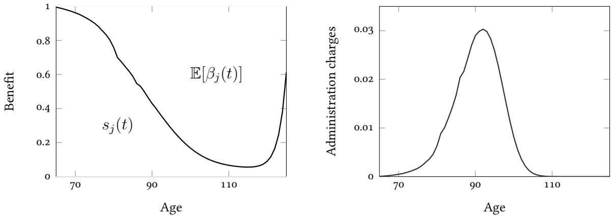
FIGURE 2. Left Panel: Separation of expected annual benefit into fixed withdrawals s_j(t, P_0) and expected mortality credits \mathbb{E}[\beta_j(t)] for contract specifications in Example 5.2.2. Right Panel: Expected administration charges over the contract duration.
