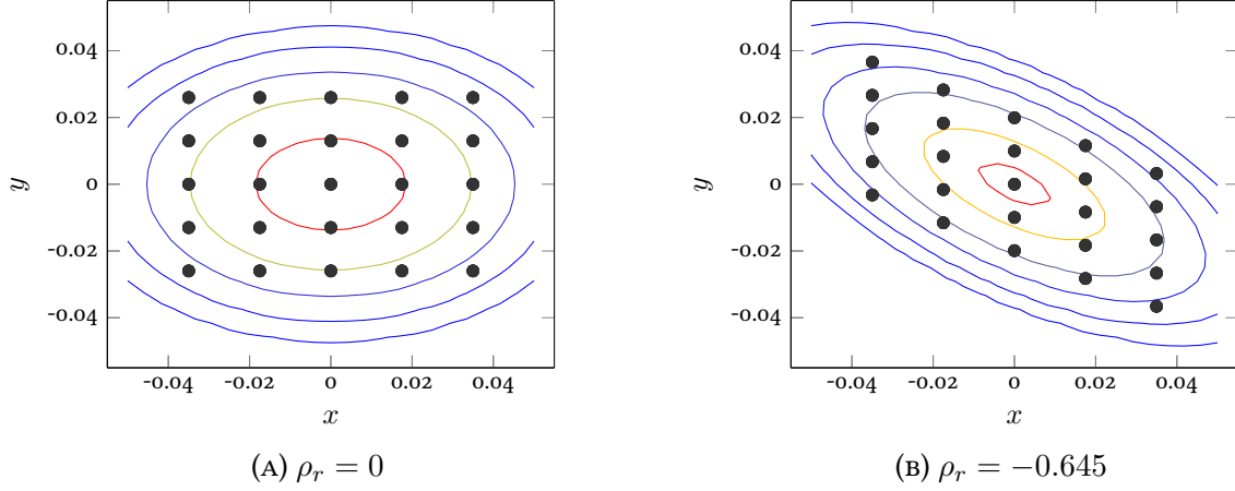
FIGURE 2. Grid points for \delta = 2 , N = 5 and different levels of \rho_r in black. Coloured lines represent contour levels of the bivariate normal distribution of (x_1, y_1) . The remaining parameters are chosen as in Table 1.
