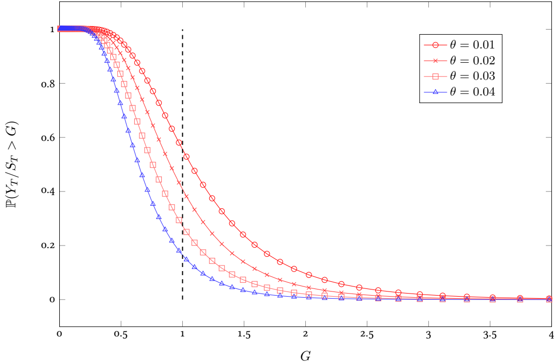
FIGURE 3. Probability that the ratio between the terminal payoff and the value of the underlying at maturity Y_T/S_T exceeds thresholds G for different values of the long-term mean \theta . The dashed line at G = 1 marks the probability of being underfunded. The remaining parameters have been chosen as in Table 1.
