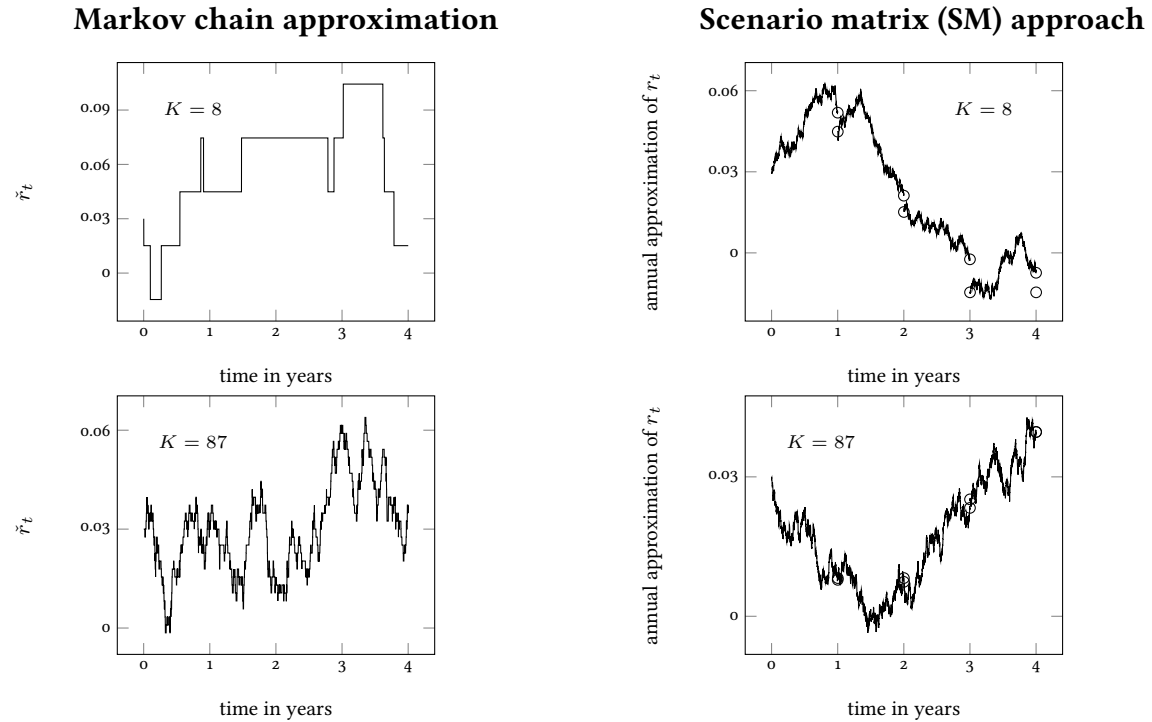
FIGURE 1. Sample paths of Markov chain approximations \tilde{r} (left column) and annual rounding to the nearest grid point as in the SM method (right column) for K = 8 (first row) and K = 87 grid points (second row). The parameters have been chosen as in Table 1.
