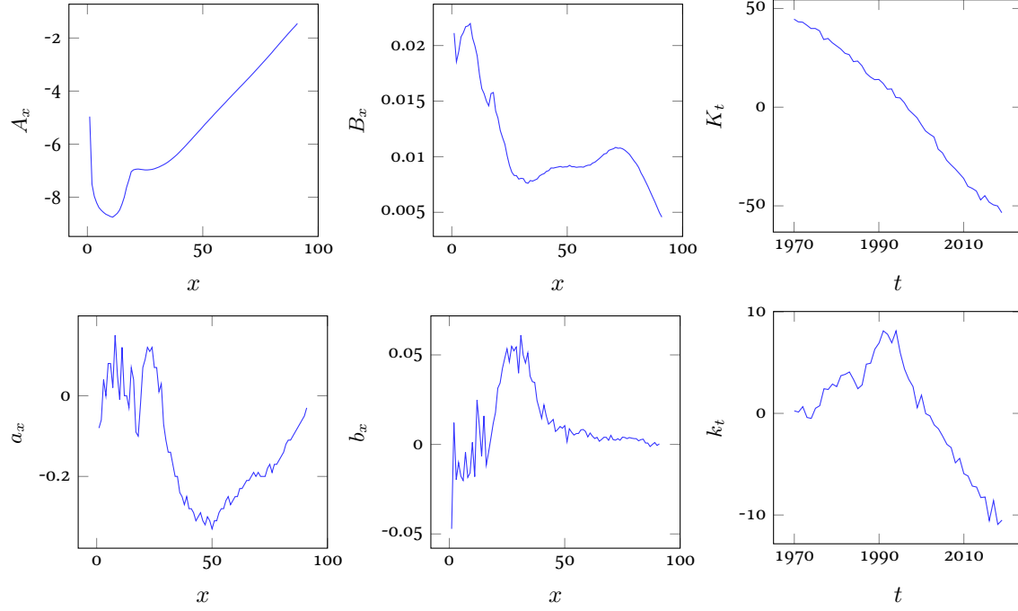
FIGURE 3. Li-Lee parameters A_x , B_x , K_t for the North-Western European population and a_x , b_x , k_t for the Swiss deviation.
