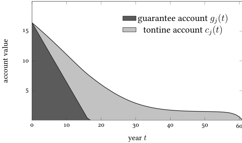
FIGURE 1. Decomposition of the total funds at time t into tontine account c_j(t) and guarantee account g_j(t) for guarantee level \alpha = 100\% .
