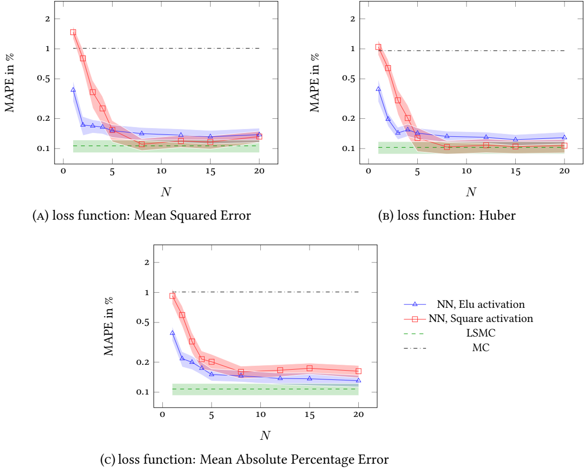
FIGURE 1. Relative error of the MC simulations and the LSMC and Neural Network algorithms as a function of the number of neurons N in the hidden layer for different activation functions and loss functions. Corresponding 95% confidence intervals in shaded colours.
