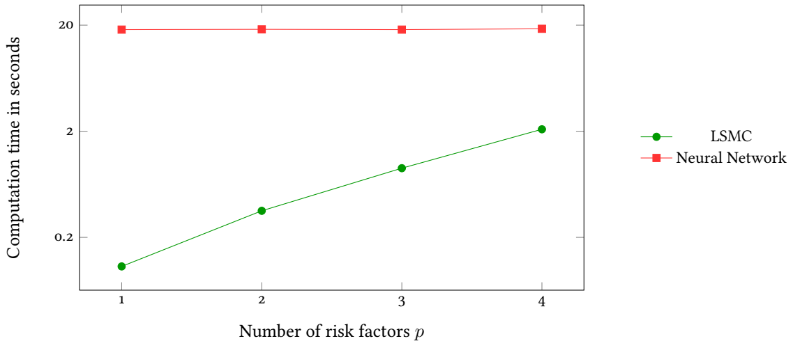
FIGURE 2. The computation time in seconds spent on running the LSMC algorithm and the neural network algorithm for 100 epochs in relation to the number of risk factors p .
