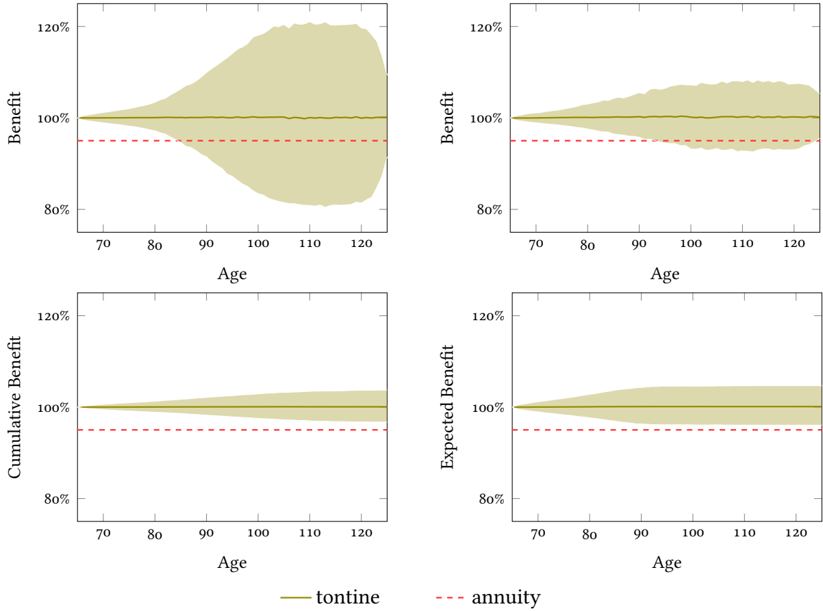
FIGURE 6. Top: Mean annual benefit of a tontine member, with guarantee level \alpha = 100\% and initial investment P_0 = 100\,000 in a tontine pool accepting n = 100 (left) and n = 1\,000 (right) members per year. Bottom Left: Mean cumulative benefit of the same individual up to every age. Bottom Right: Mean expected benefits b^* for the same person computed in the update step in Algorithm 3.
