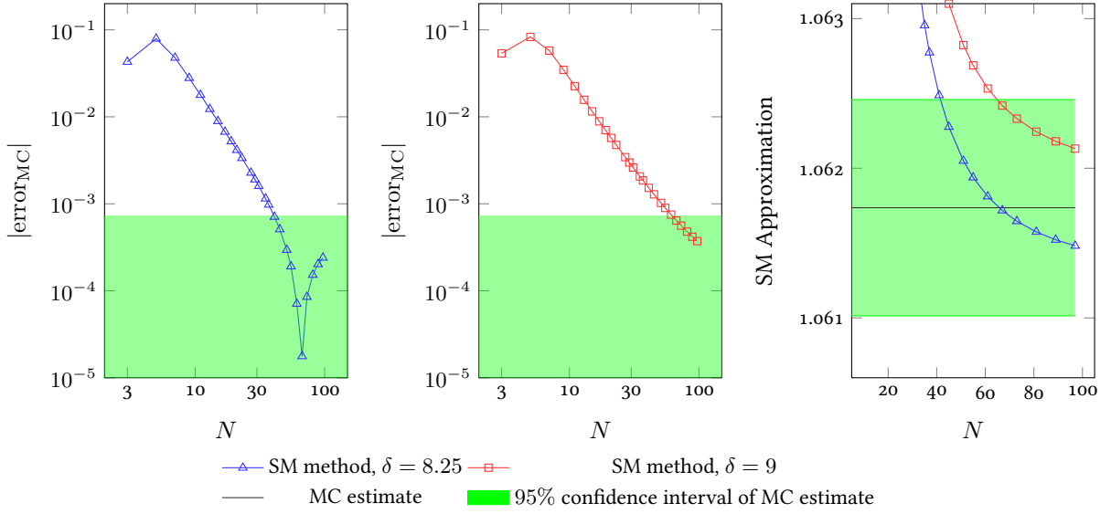
FIGURE 3. Panels 1 and 2: Error as a function of the number of grid points for different values of parameter \delta that determines the width of the discretisation interval as in Equation (41). Panel 3: Approximation via scenario-matrix method as a function of the number of grid points N in blue and red compared to the approximation via Monte-Carlo simulation in black. Shaded green: 95%-confidence interval of Monte-Carlo simulation. The parameters are chosen as in Table 1.
