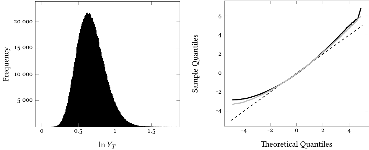
FIGURE 4. Histogram and quantile-quantile plot of the logarithm of the final payoff \ln Y_T . Stochastic interest rates in black, constant interest rates in grey. Samples from Monte-Carlo simulations with 10^6 scenarios. The parameters are chosen as in Table 1.
